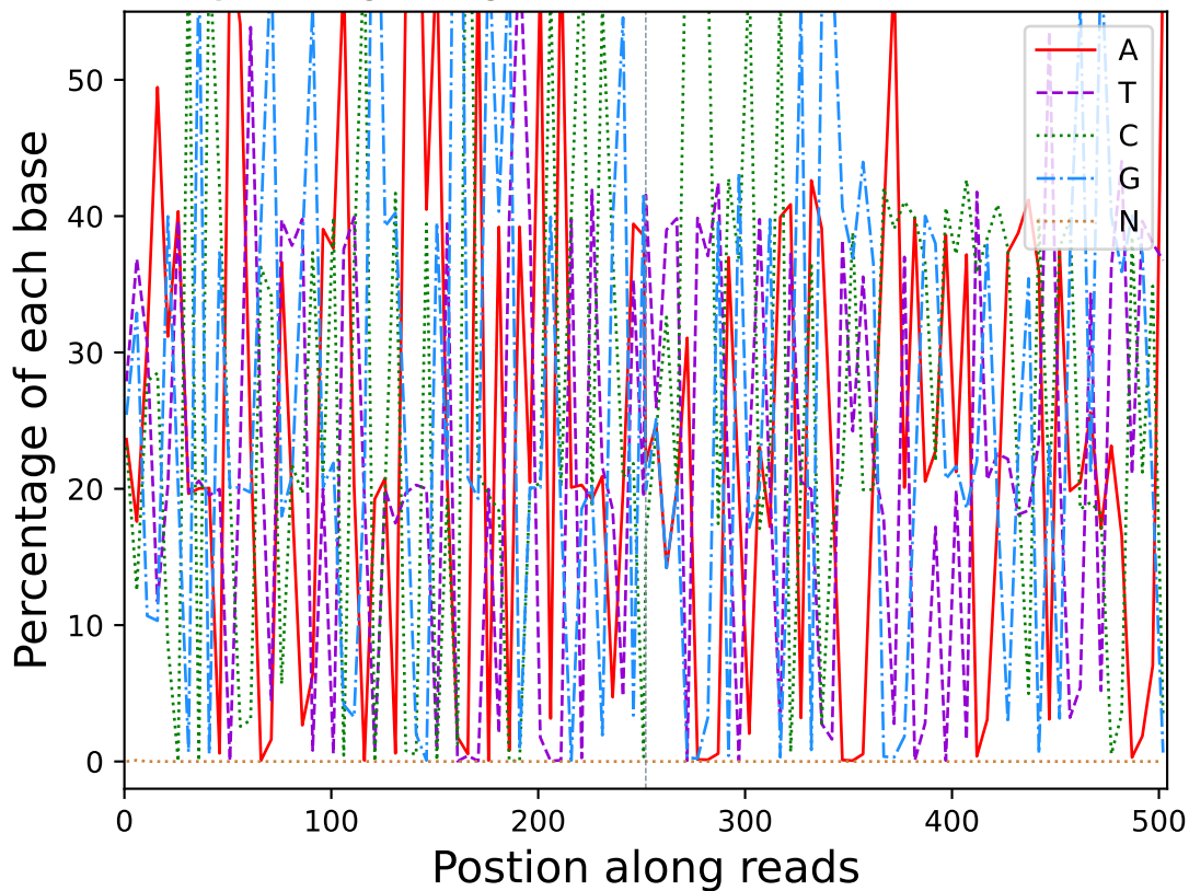
Base percentage along reads (R10403)
